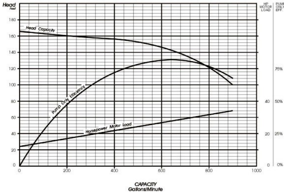
Pump Performance Curve for RWN700A 1 stage @ 2900 RPM; Sp Gr = 1
