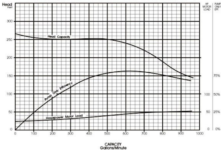
Pump Performance Curve for RWN700A 1 stage @ 3450 RPM; Sp Gr = 1
