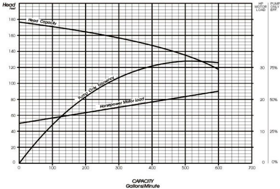
Pump Performance Curve for RWN575A 1 stage @ 2900 RPM; Sp Gr = 1
