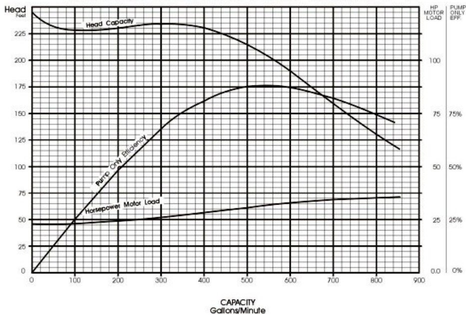
Pump Performance Curve for RWN575A 1 stage @ 3450 RPM; Sp Gr = 1
