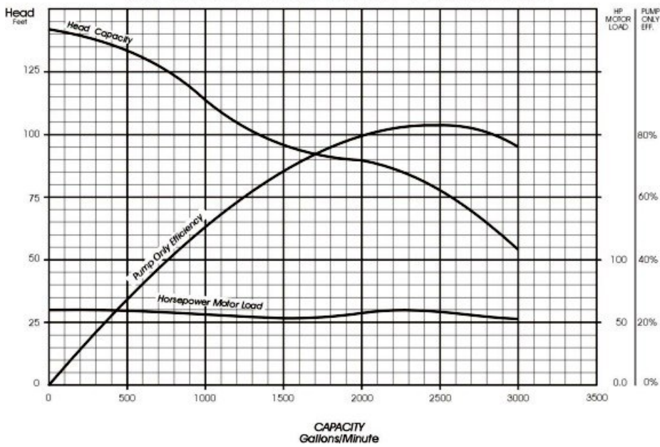
Pump Performance Curve for RWN2900A 1 stage @ 2900 RPM
