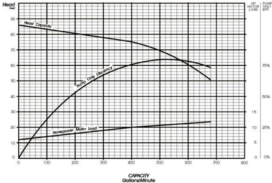
Pump Performance Curve for RWM575A 1 stage @ 2900 RPM; Sp Gr = 1
