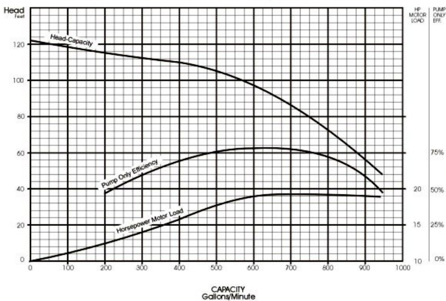
Pump Performance Curve for RWM575A 1 stage @ 3450 RPM; Sp Gr = 1
