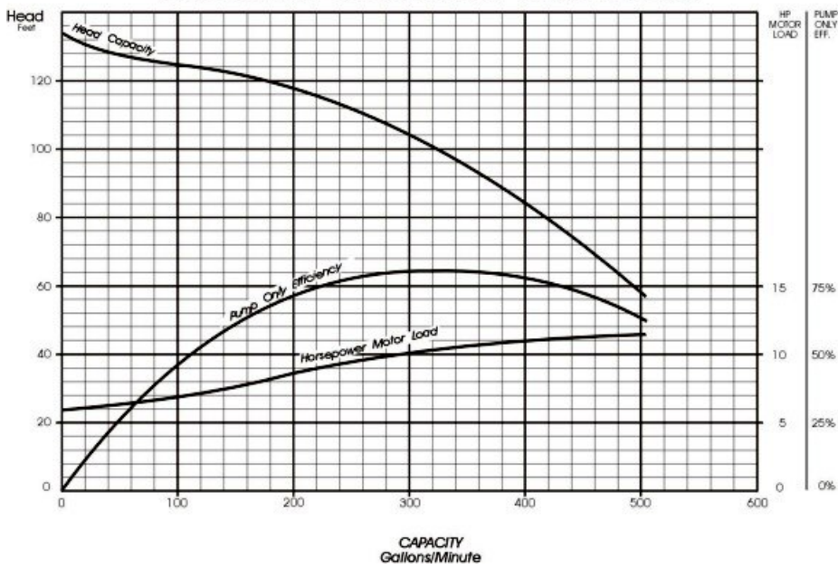
Pump Performance Curve for RWM400A 1 stage @ 3450 RPM
