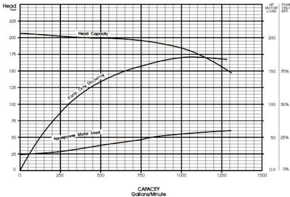
Pump Performance Curve for RWM1100A 1 stage @ 3450 RPM; Sp Gr = 1
