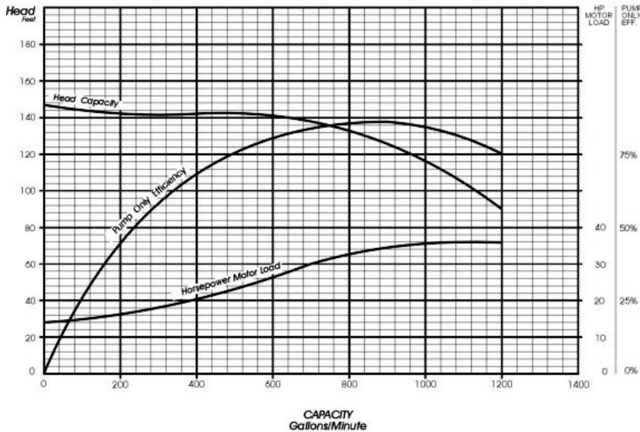
Pump Performance Curve for RWM1100A 1 stage @ 2900 RPM; Sp Gr = 1
