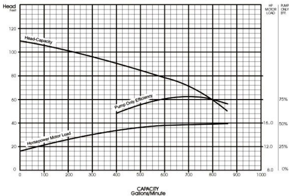
Pump Performance Curve for RWJ700A 1 stage @ 3450 RPM; Sp Gr = 1
