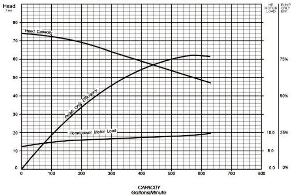
Pump Performance Curve for RWJ700A 1 stage @ 2900 RPM
