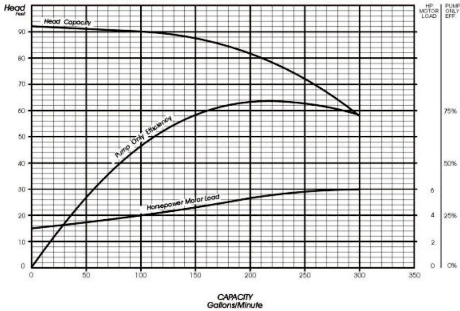
Pump Performance Curve for RWJ275A 1 stage @ 2900 RPM; Sp Gr = 1
