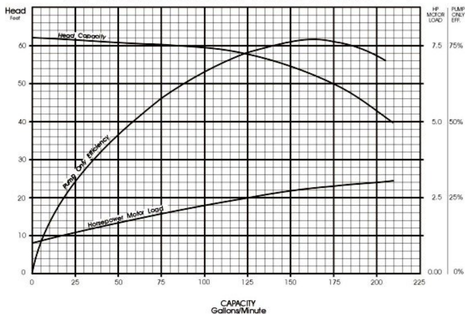
Pump Performance Curve for RWJ145A 1 stage @ 3500 RPM; Sp Gr = 1
