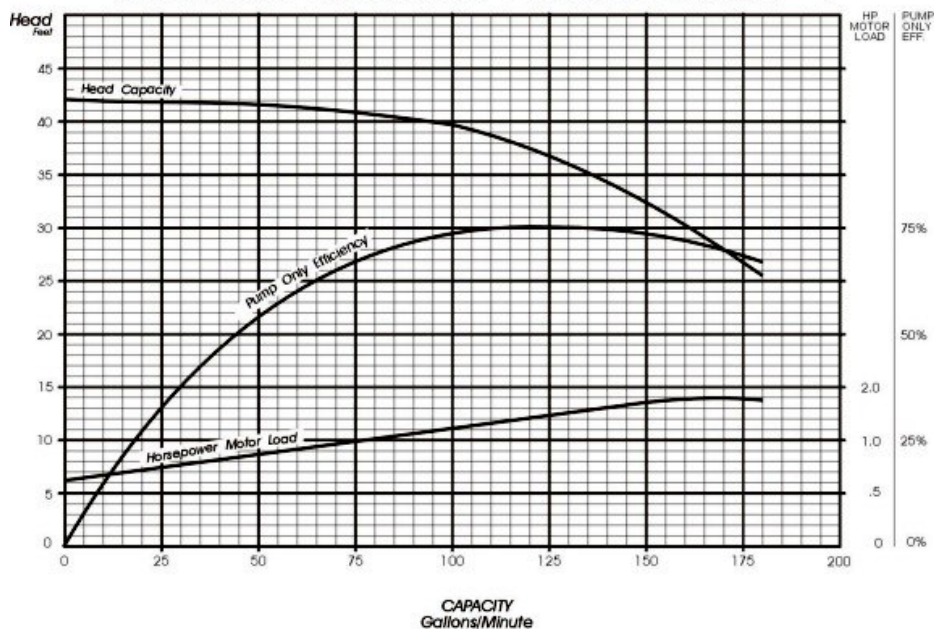
Pump Performance Curve for RWJ145A 1 stage @ 2900 RPM; Sp Gr = 1
