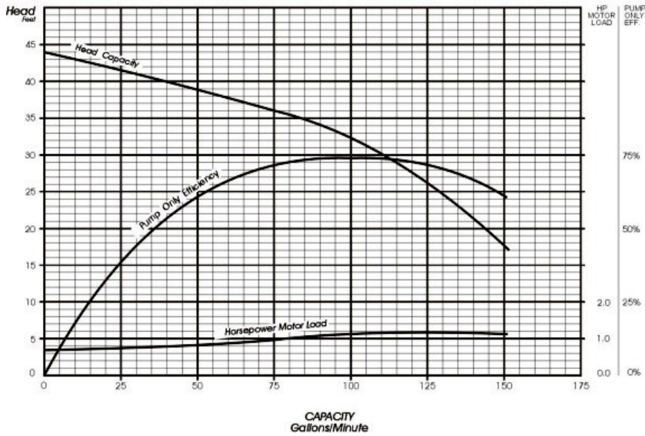
Pump Performance Curve for RWJ120A 1 stage @ 2900 RPM; Sp Gr = 1
